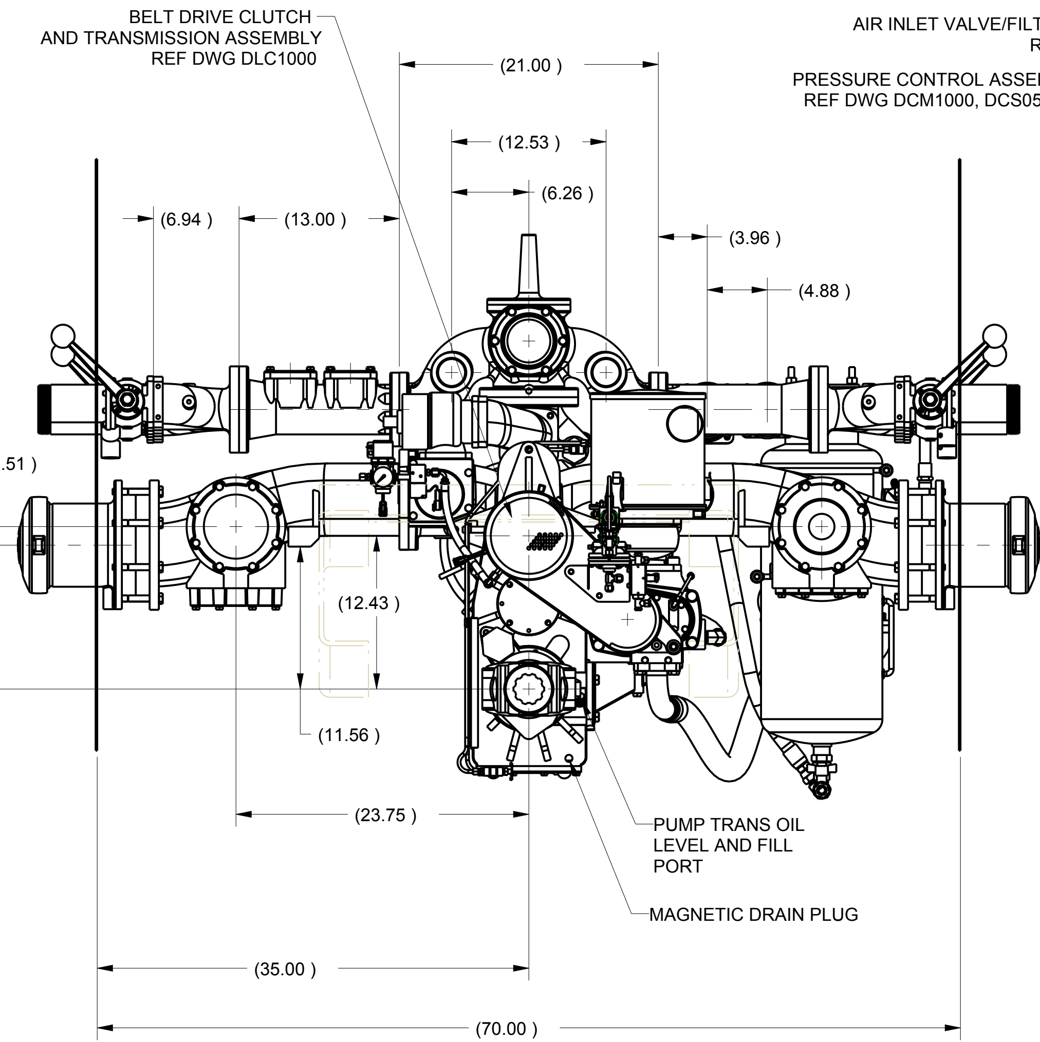
REAR VIEW
