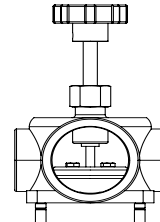
HA00313 (2) 1.5" NPT (2) 2.5" NPT
