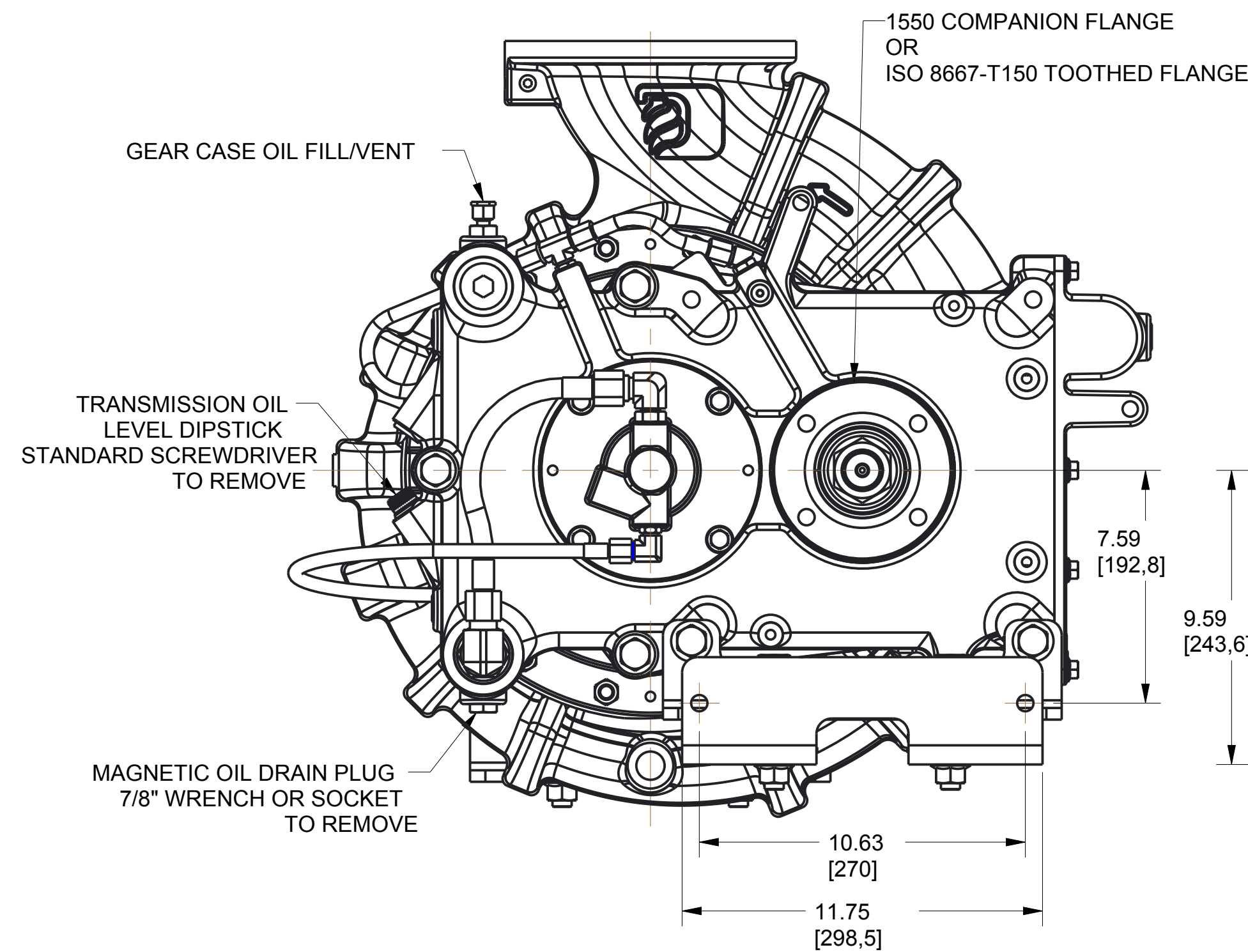
1550 COMPANION FLANGE
