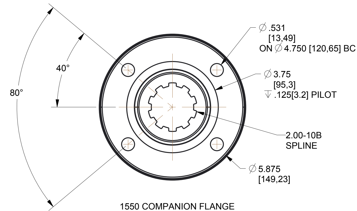
1550 COMPANION FLANGE
