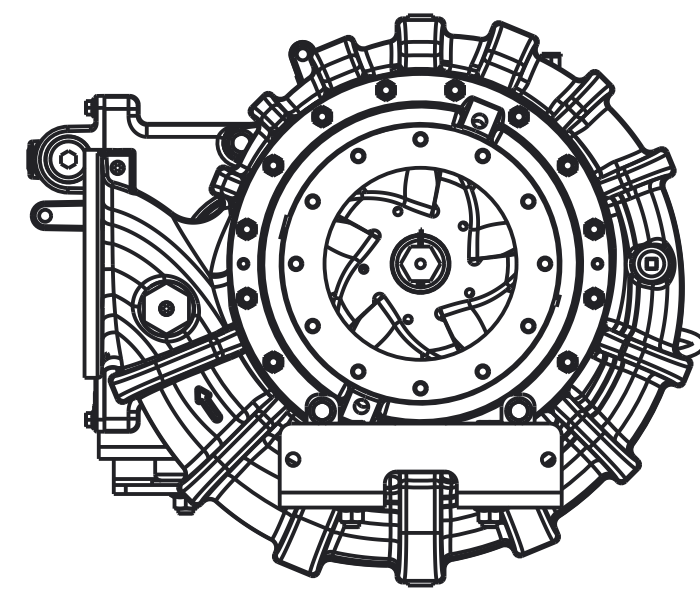
9 O'CLOCK DISCHARGE
