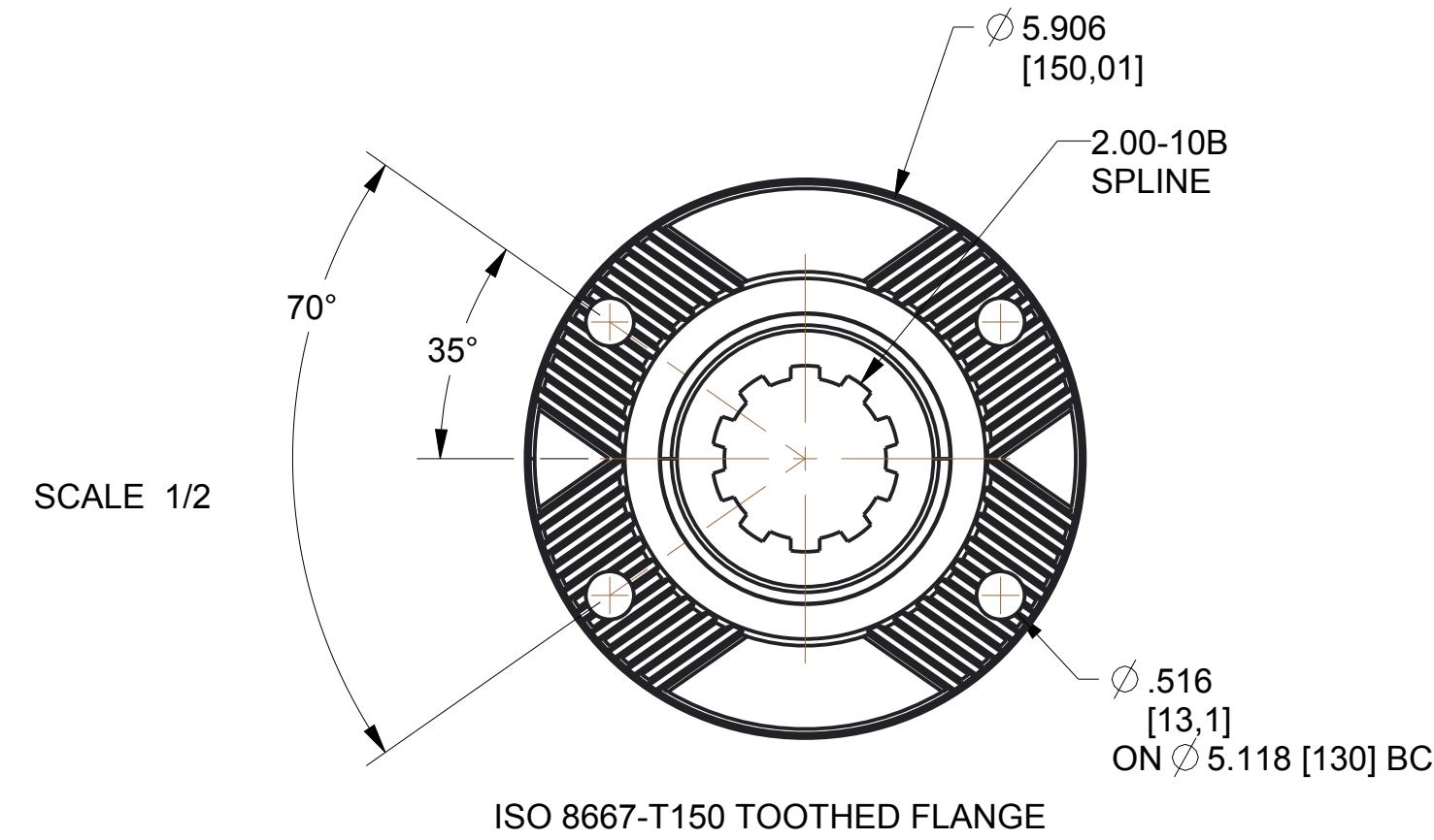
ISO 8667-T150 TOOTHED FLANGE
