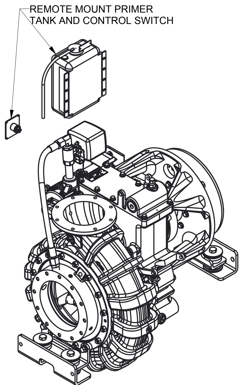
STANDARD 12 O'CLOCK DISCHARGE SCALE 1/8
