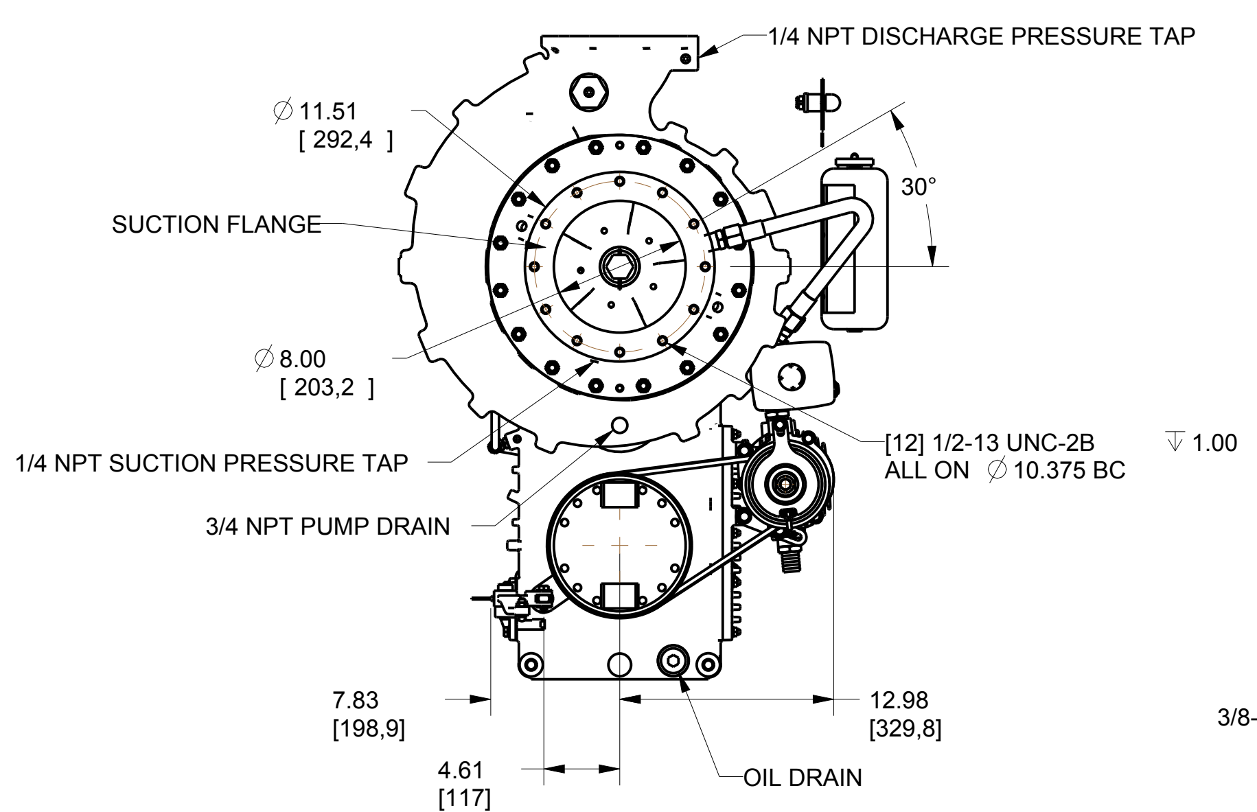
VIEW FROM THE ENGINE TO THE PUMP
