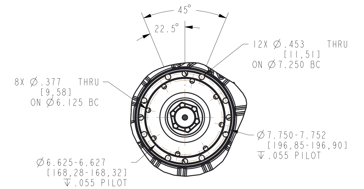
COMPANION FLANGE DETAIL SCALE 1/4
