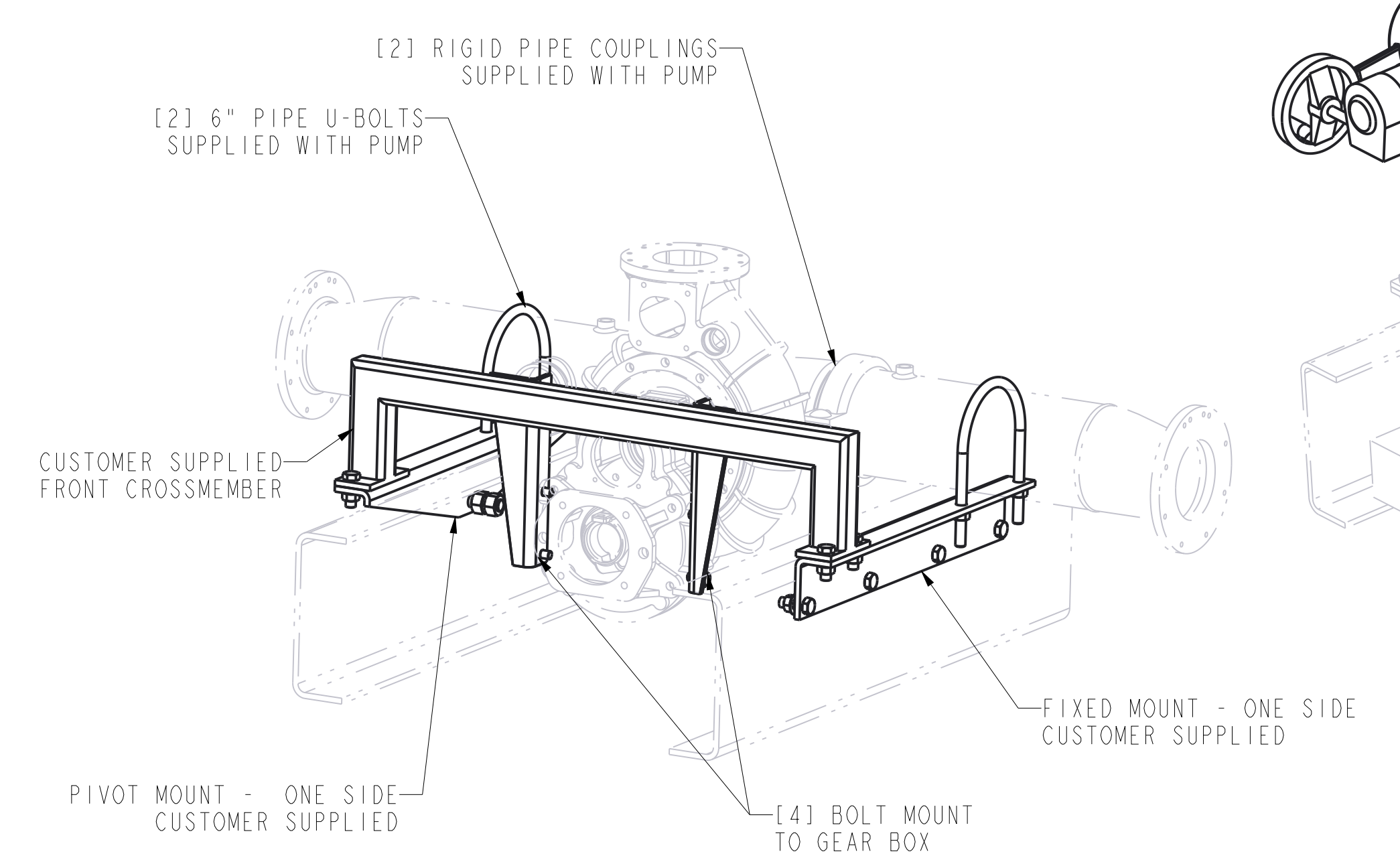
SUGGESTED MOUNT CONFIGURATION SCALE 1/8
