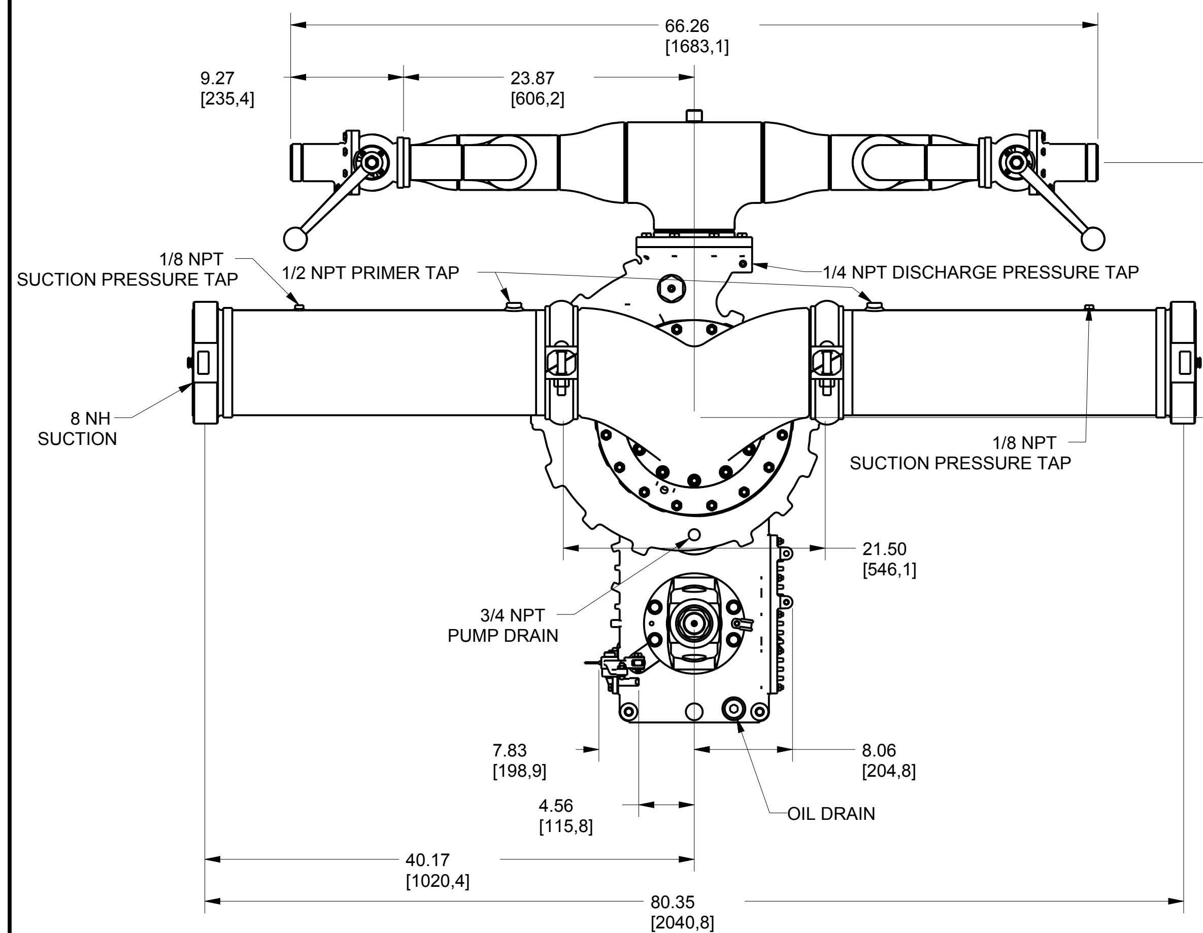
VIEW FROM THE ENGINE TO THE PUMP
