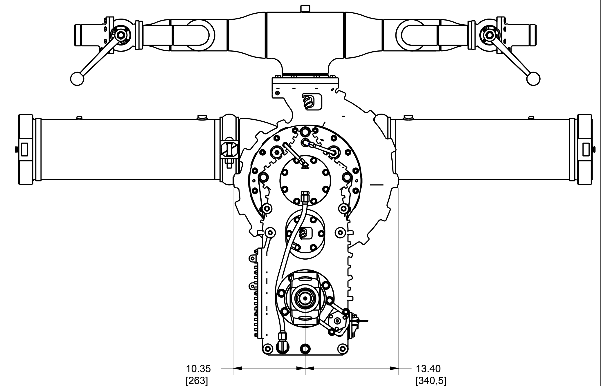
VIEW FROM THE PUMP TO THE ENGINE
