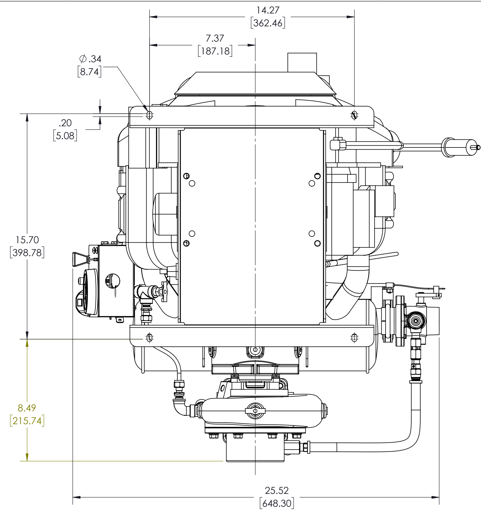
BOTTOM VIEW
