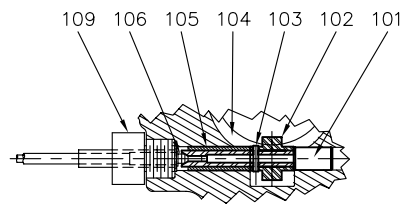
TACH. DETAIL
